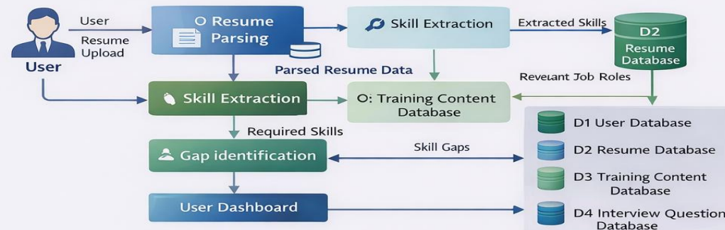
Level 2 DFD (Resume Analysis Module)
